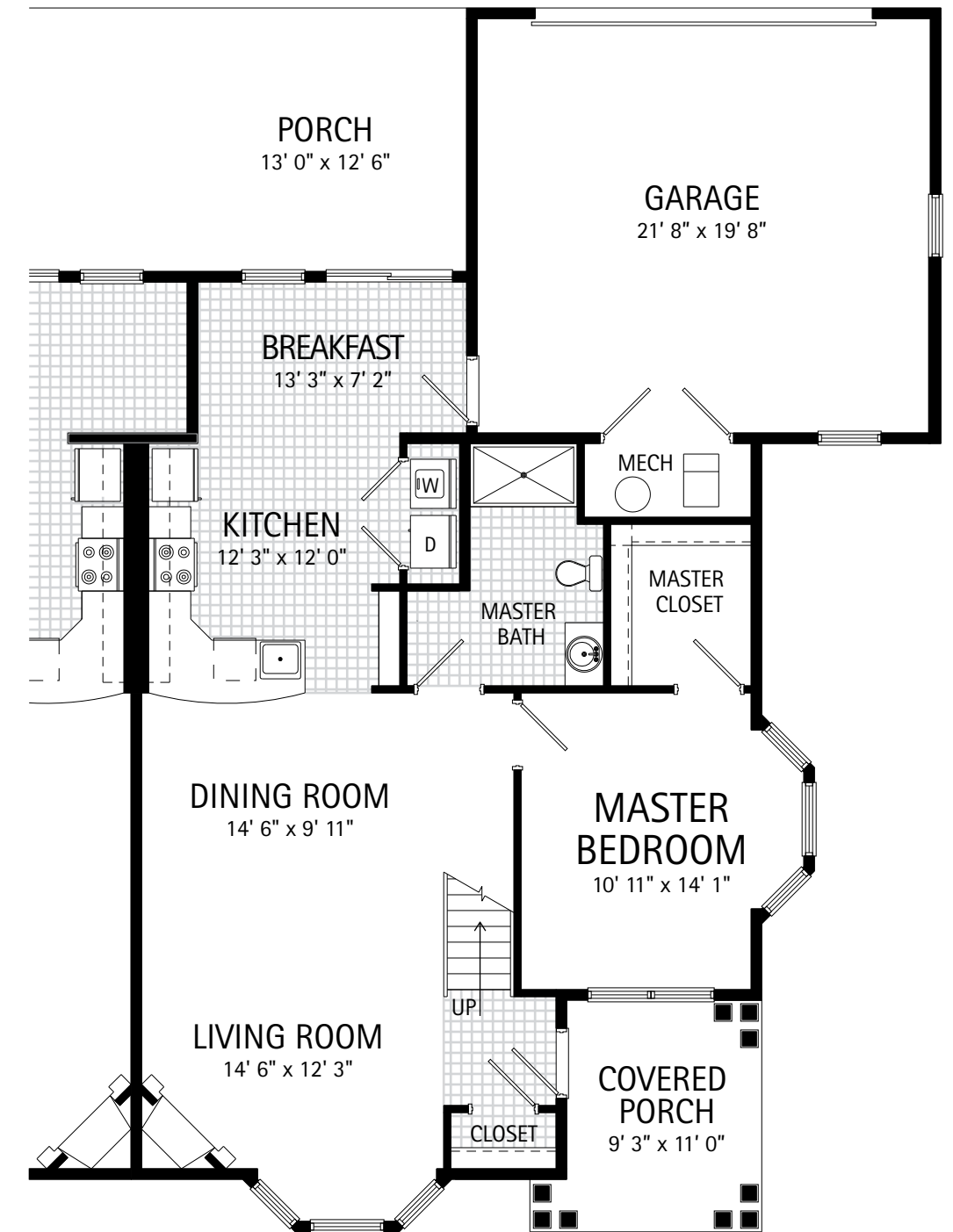
FIRST FLOOR - 1,019 S.F.
