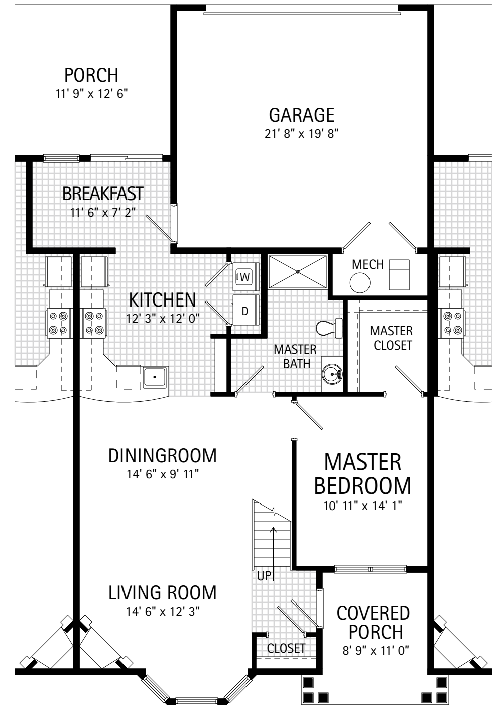
FIRST FLOOR - 898 S.F.
