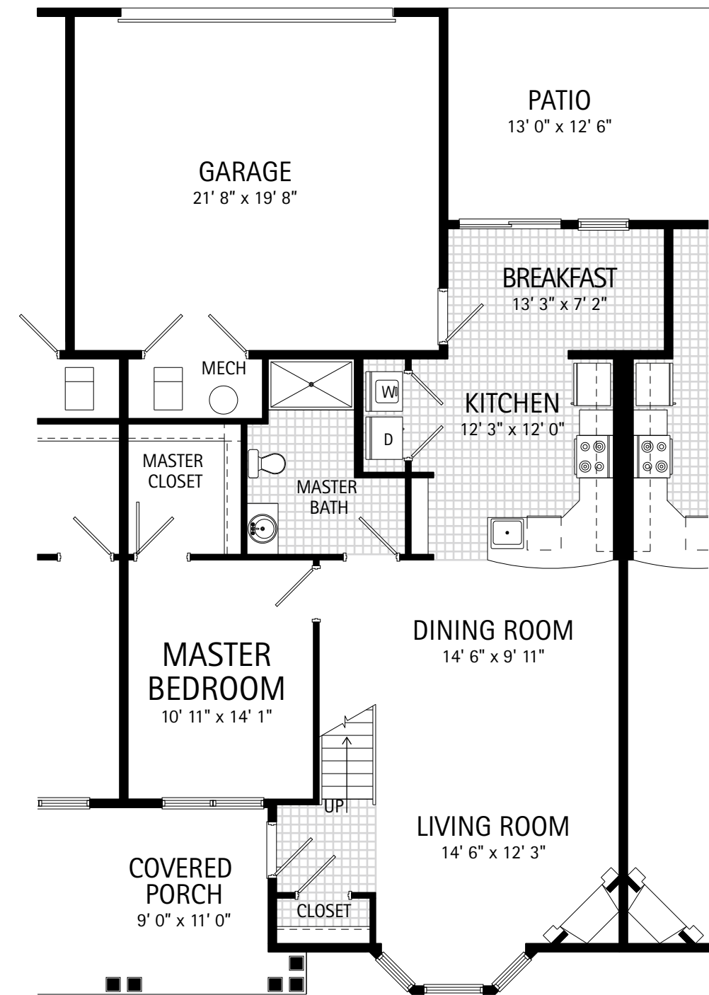
FIRST FLOOR - 906 S.F.
