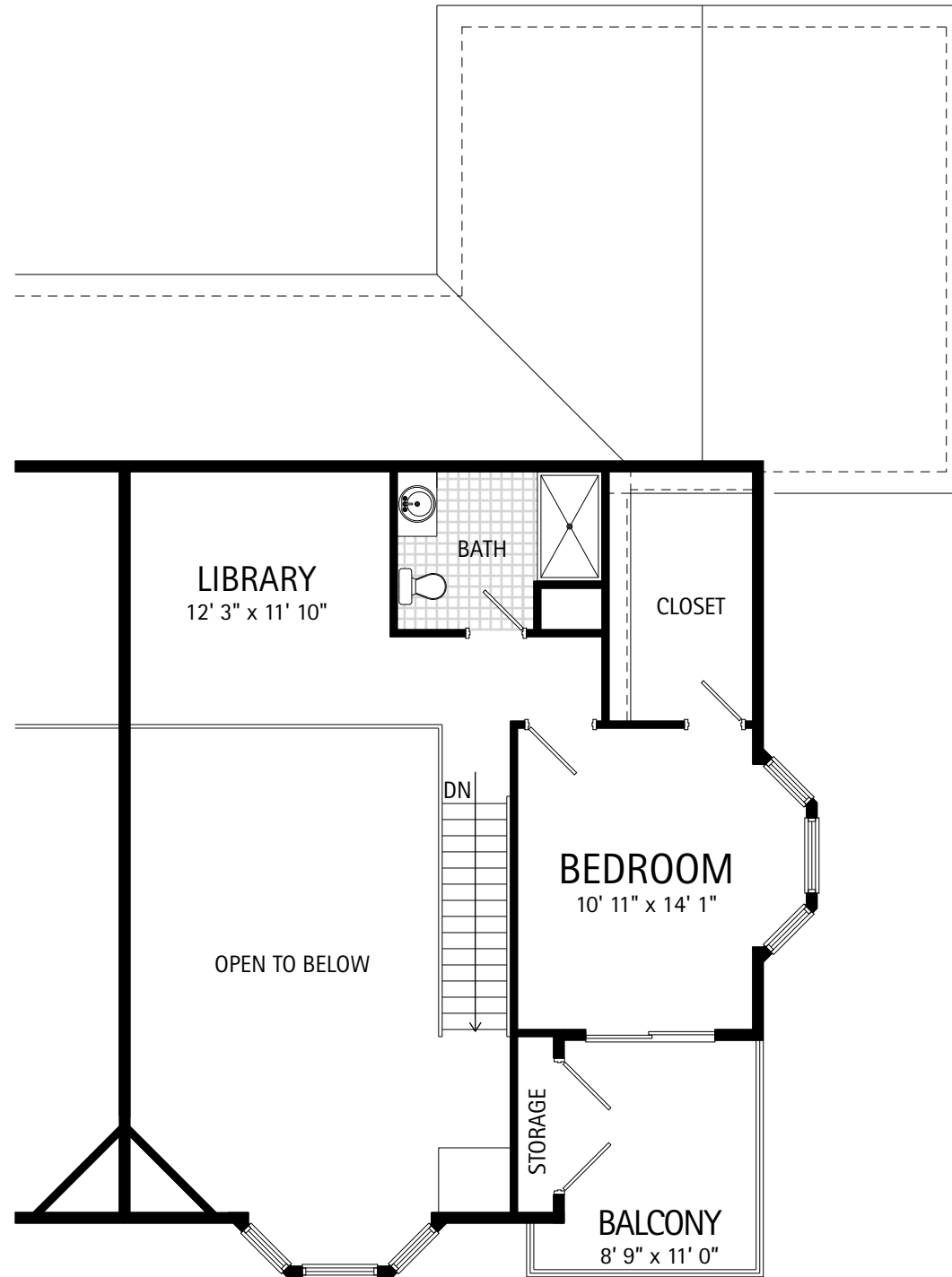
SECOND FLOOR - 584 S.F.
